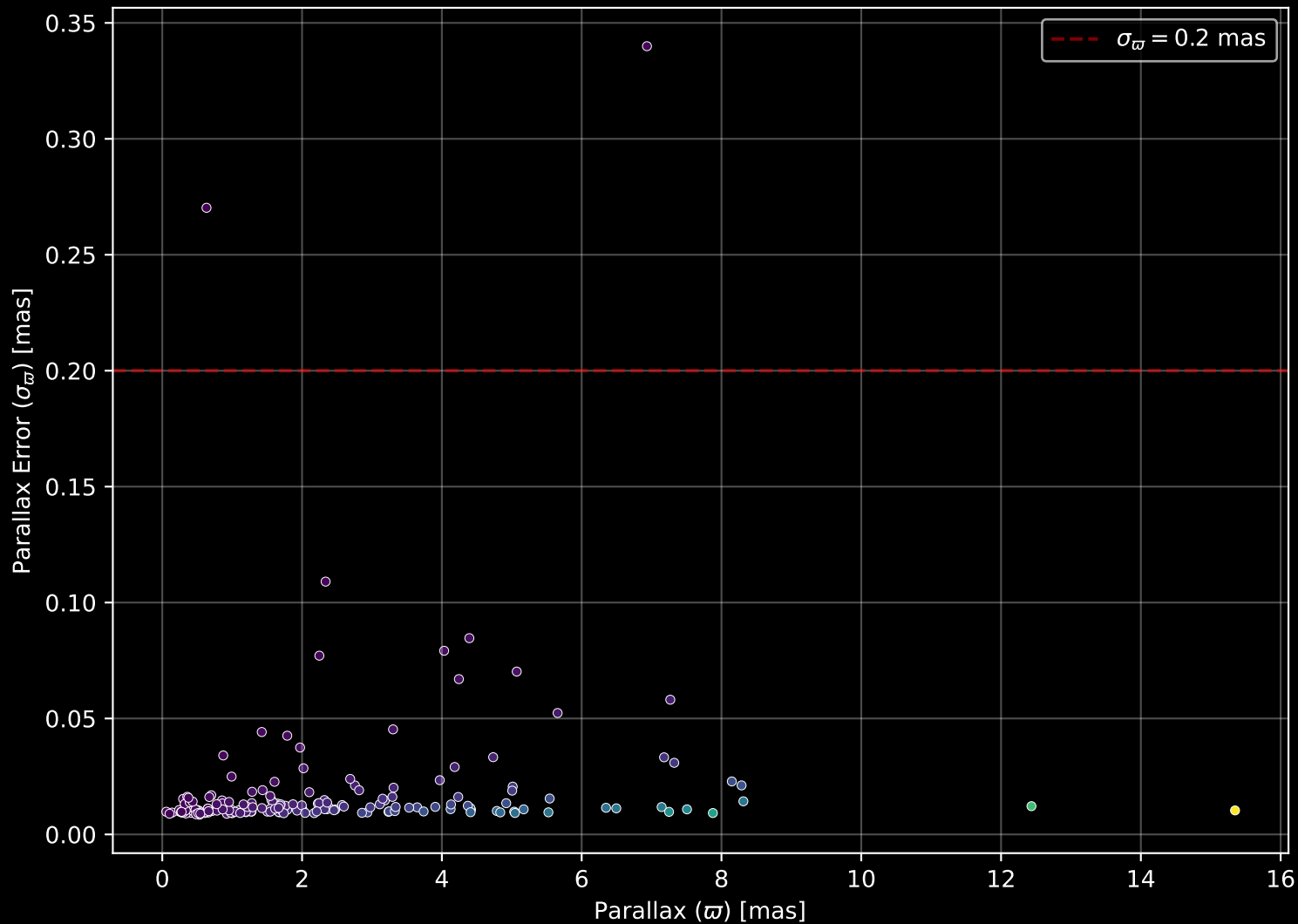
APOGEE DR17 Field: [267-29-O_TESS] Parallax Quality (n= 187)
