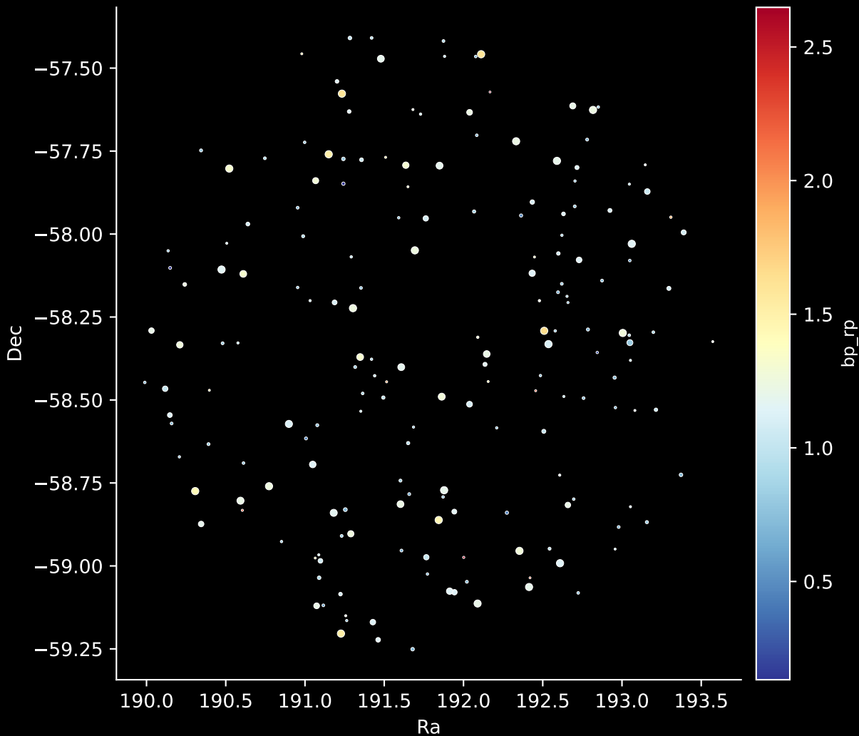
APOGEE DR17 Field: [267-29-O_TESS] Stars: 187
