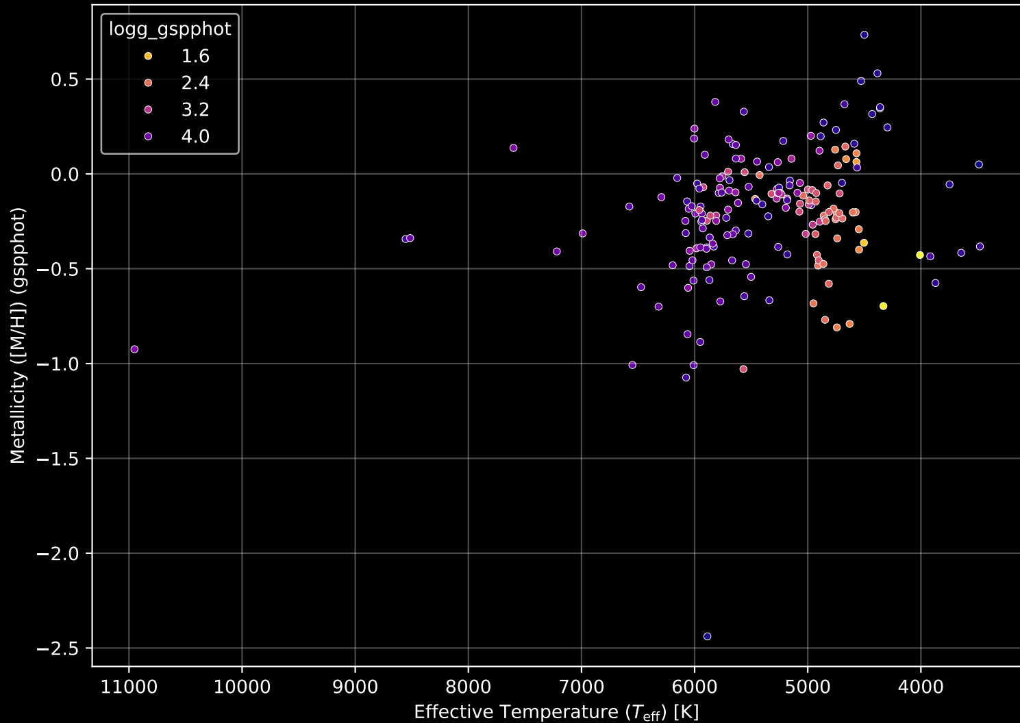
APOGEE DR17 Field: [267-29-O_TESS] Stellar Population Parameters (n= 187)
