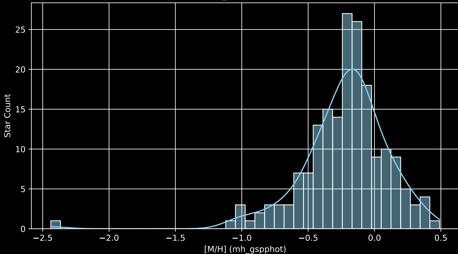
APOGEE DR17 Field: [267-29-O_TESS [M/H] (mh_gspphot) (n= 185)
