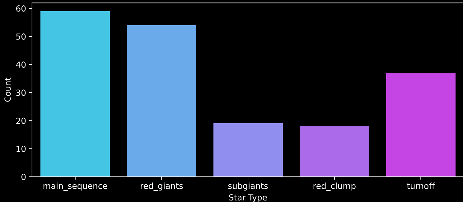
APOGEE DR17 Field: [267-29-O_TESS] Count plot of Star Type
