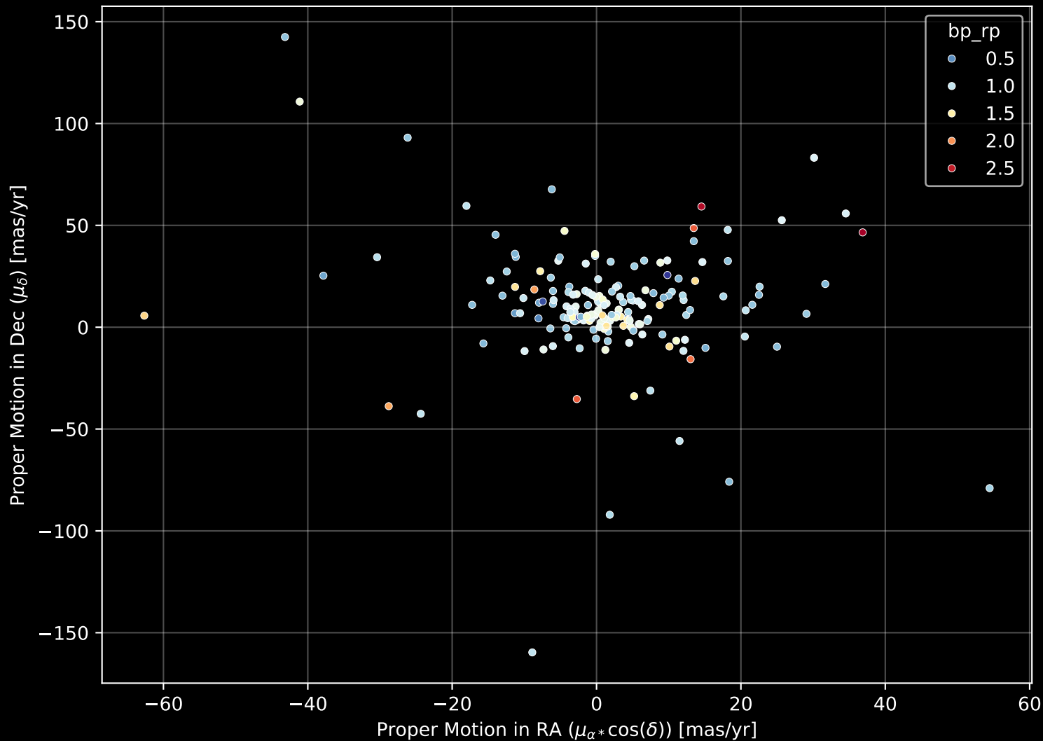
APOGEE DR17 Field: [267-29-O_TESS] Proper Motion Diagram (n= 187)
