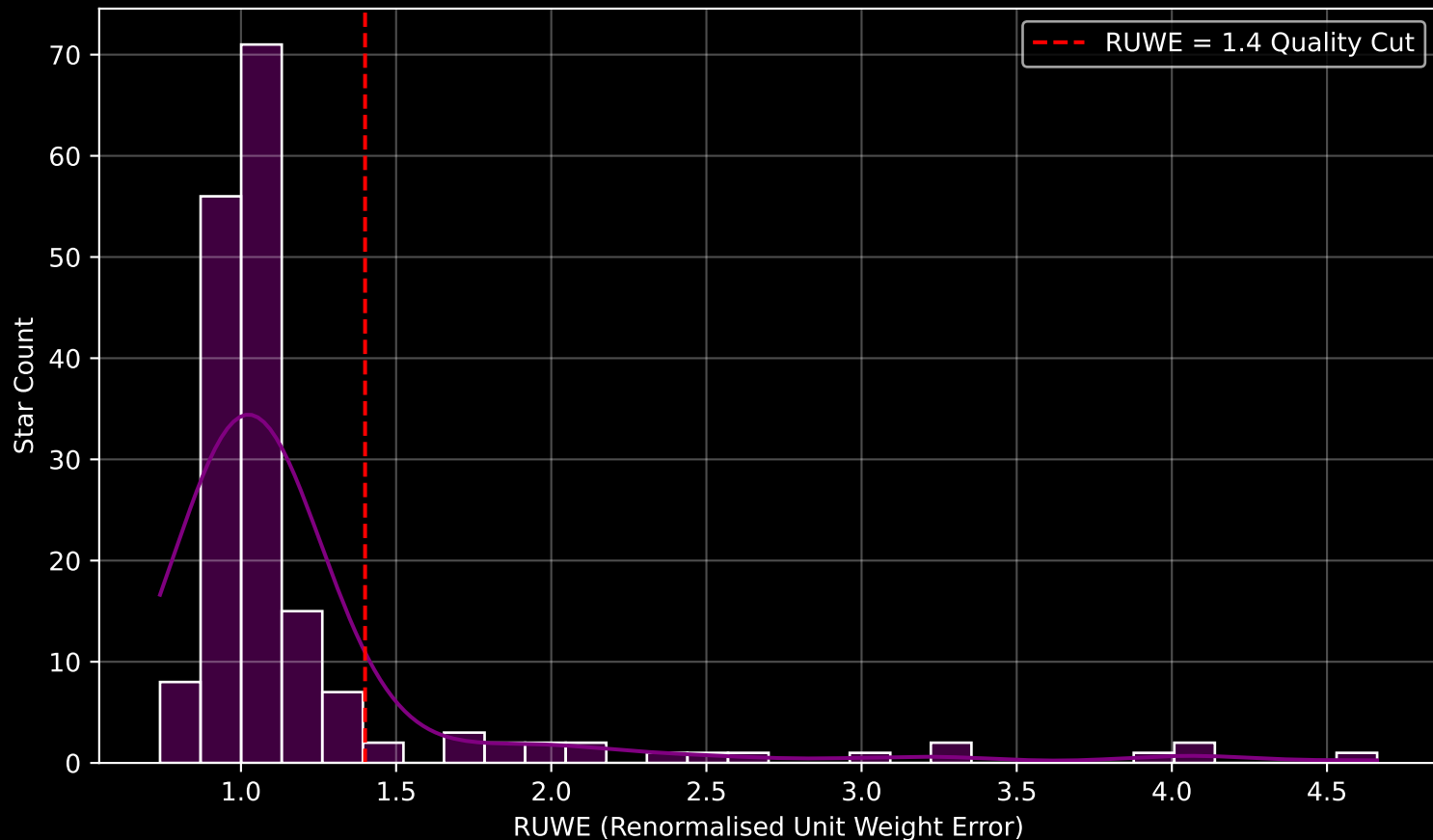
GAPOGEE DR17 Field [267-29-O_TESS] RUWE Distribution (n= 178)
