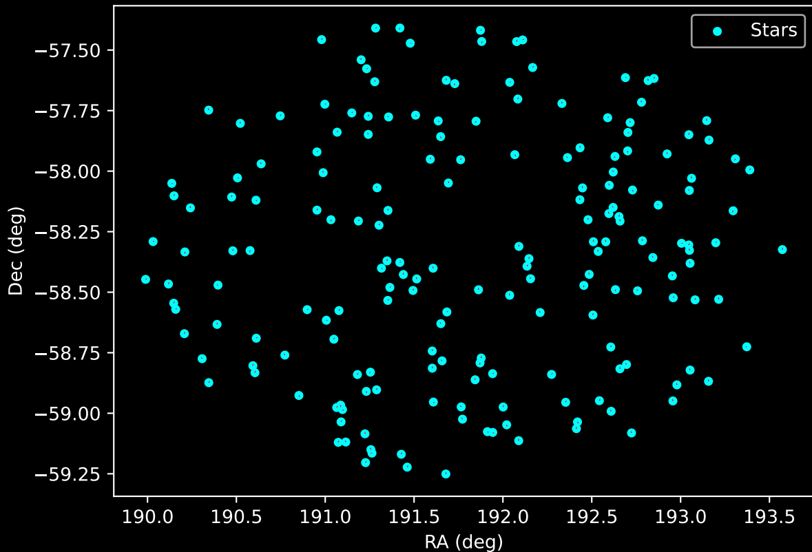
APOGEE DR17 Field: [267-29-O_TESS] Proper Motion Vectors for Gaia Star Field (n= 187)
